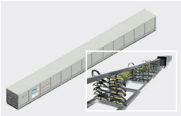
ROLL-ON / ROLL-OFF SYSTEMS FOR VERY LONG FRAMEWORK PARTS (14M STRINGER)
